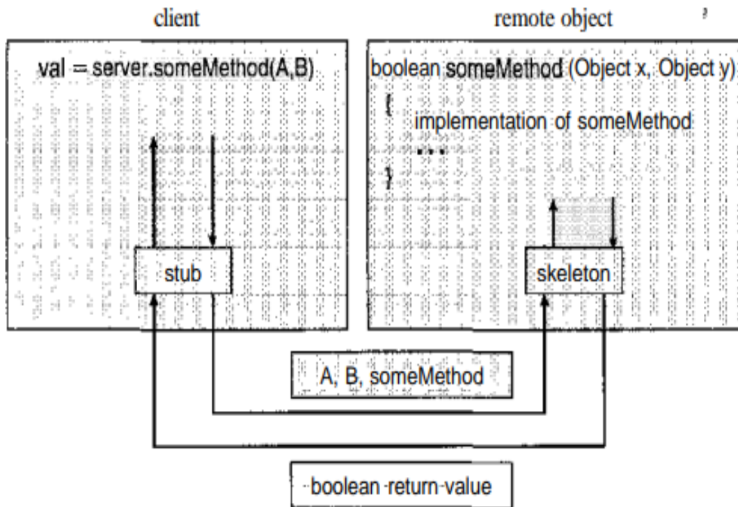
Figure 4.11 Marshalling parameters.
