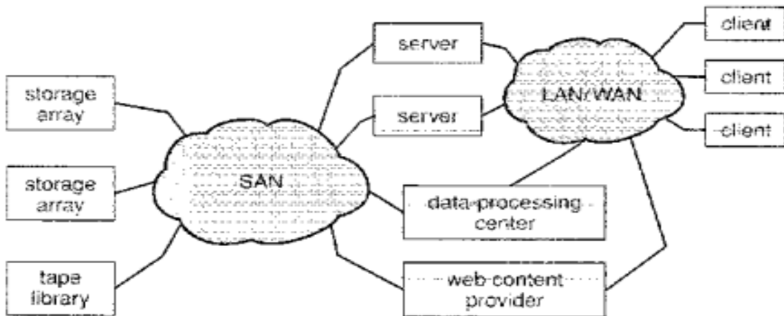
Figure 16.3 Storage-area network.
