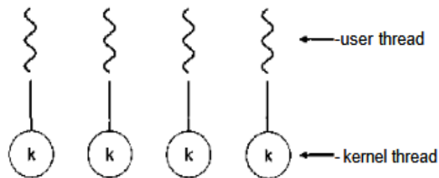
Figure 5.3 One-to-one mode
