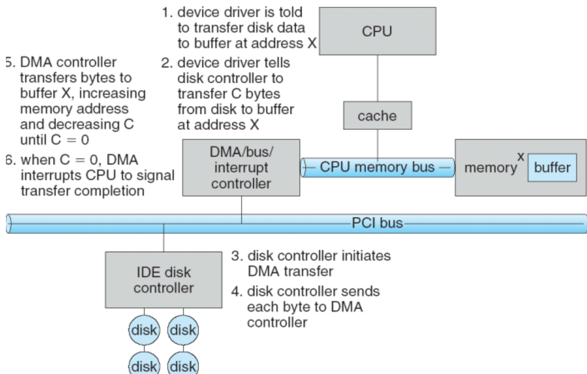
Figure 17.4 Steps in a DMA transfer.
