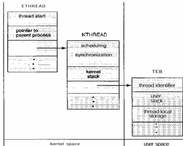
Figure 5.9 Data structures of a Windows XP thread.
