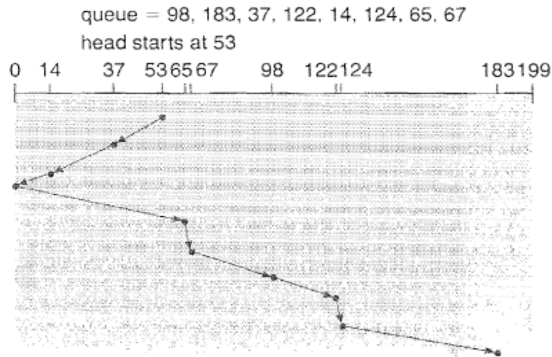
Figure 16.6 SCAN disk scheduling
