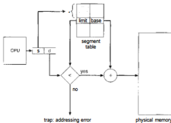
Figure 12.10 Segmentation hardware
