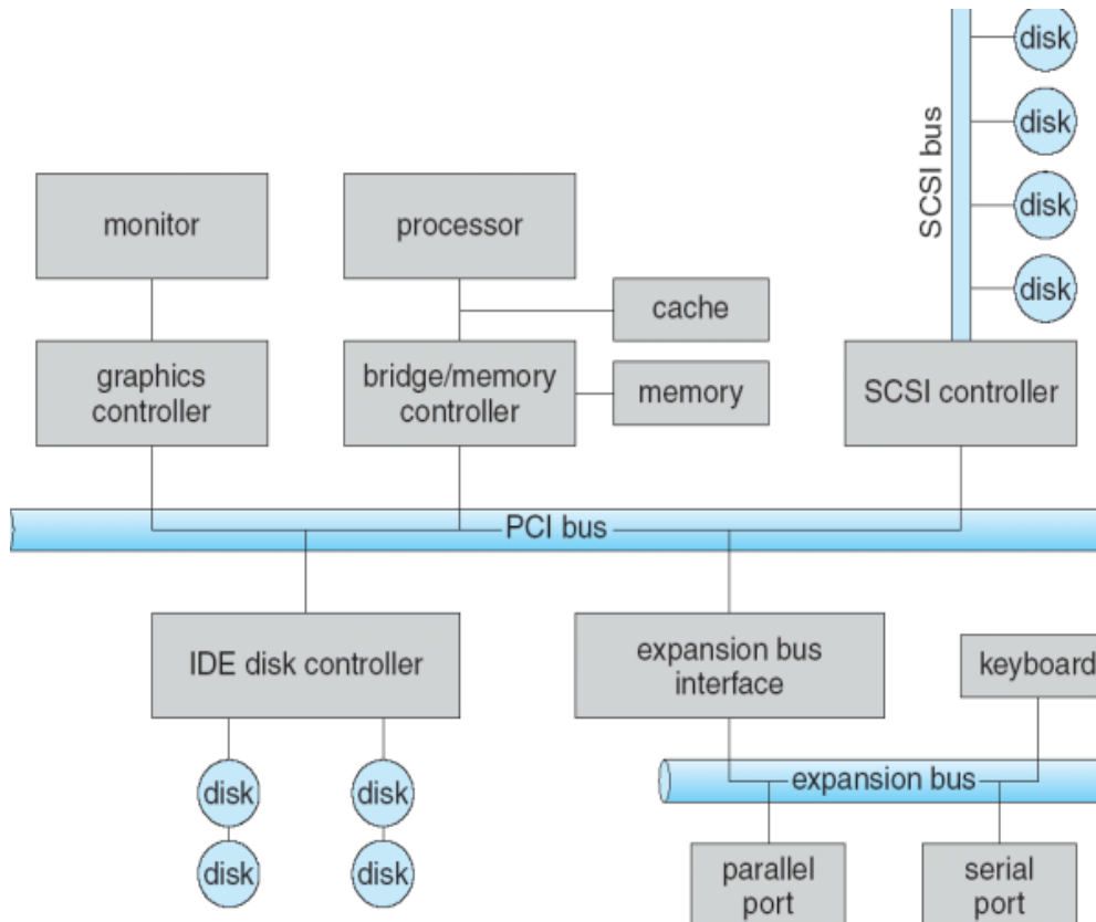
Figure 17.1 A typical PC bus Structure
