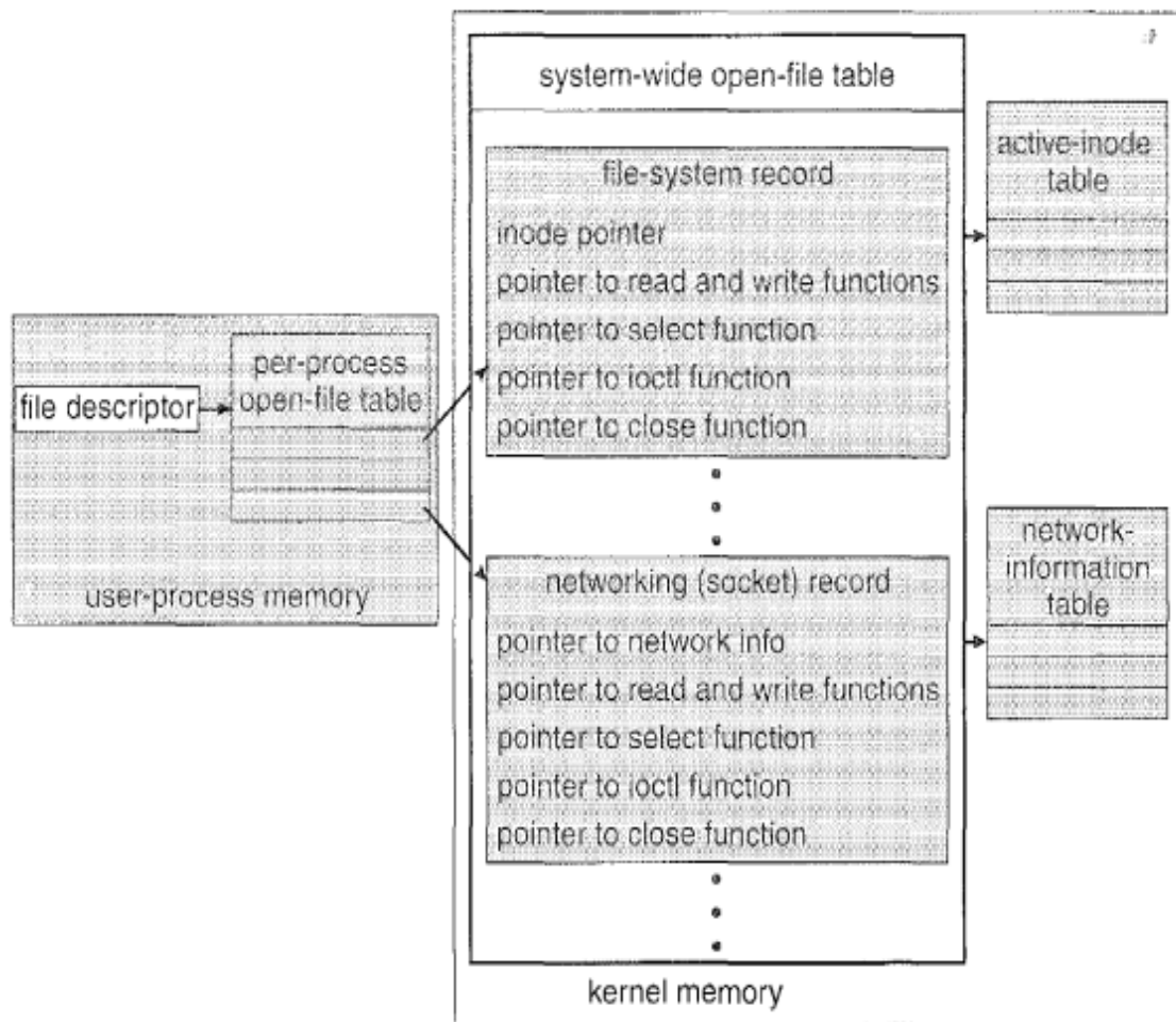
Figure 17.8 UNIX I/O kernel structure.
