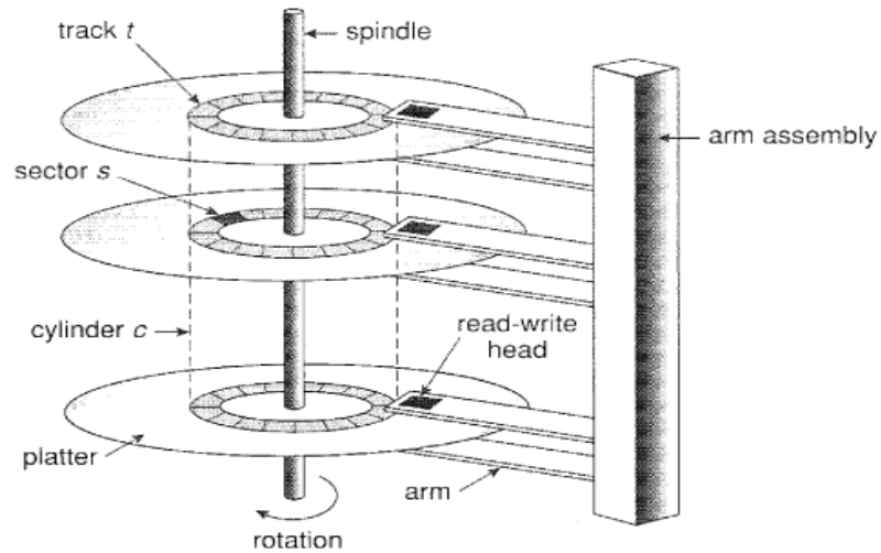
Figure 16.1 Moving-head disk mechanism.
