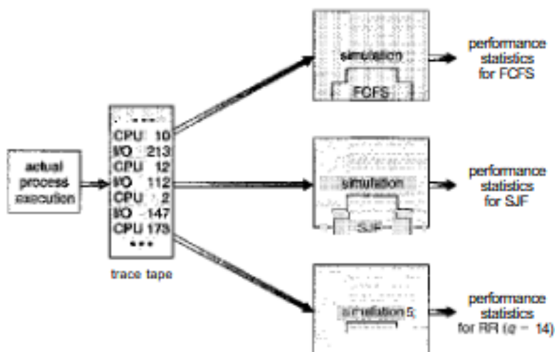
Figure 7.7 Evaluation of CPU schedulers by simulation
