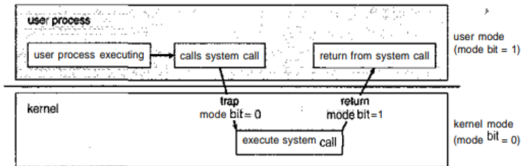
Figure 1.8 Transition from user to kernel mode.
