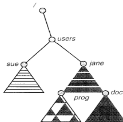
Figure 14.10 Mount point.
