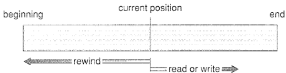
Figure 14.1 Sequential-access file
