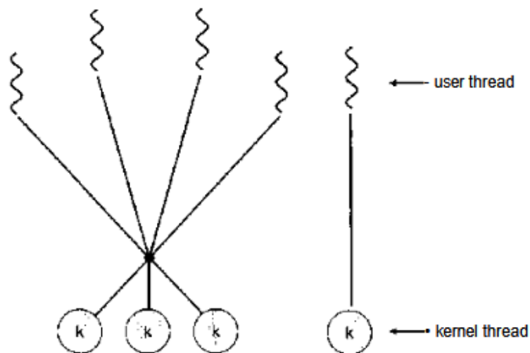
Figure 5.4 Two-level model
