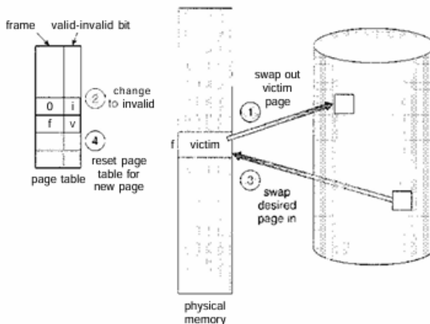
Figure 13.10 Page replacement
