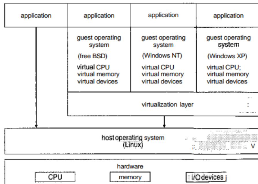
Figure 2.15 VMware Architecture
