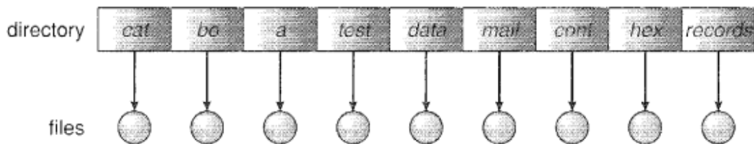
Figure 14.4 Single-level directory.
