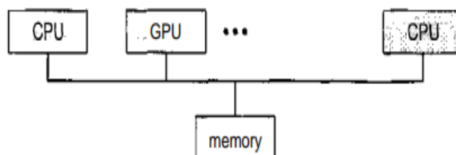
Figure 1.6 Symmetric multiprocessing architecture
