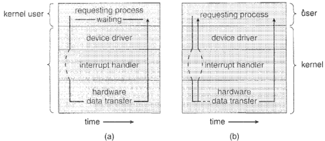
Figure 17.6 Two I/O methods: (a) synchronous and (b) asynchronous
