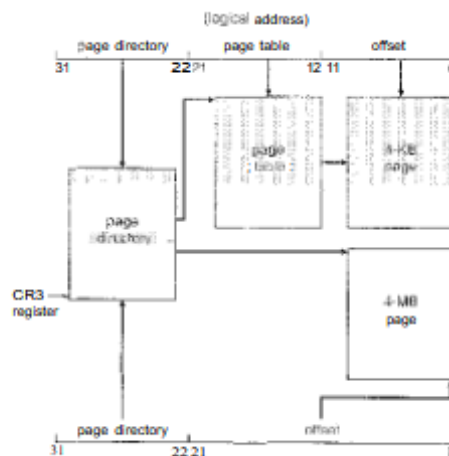
Figure 12.13 Paging in the Pentium architecture
