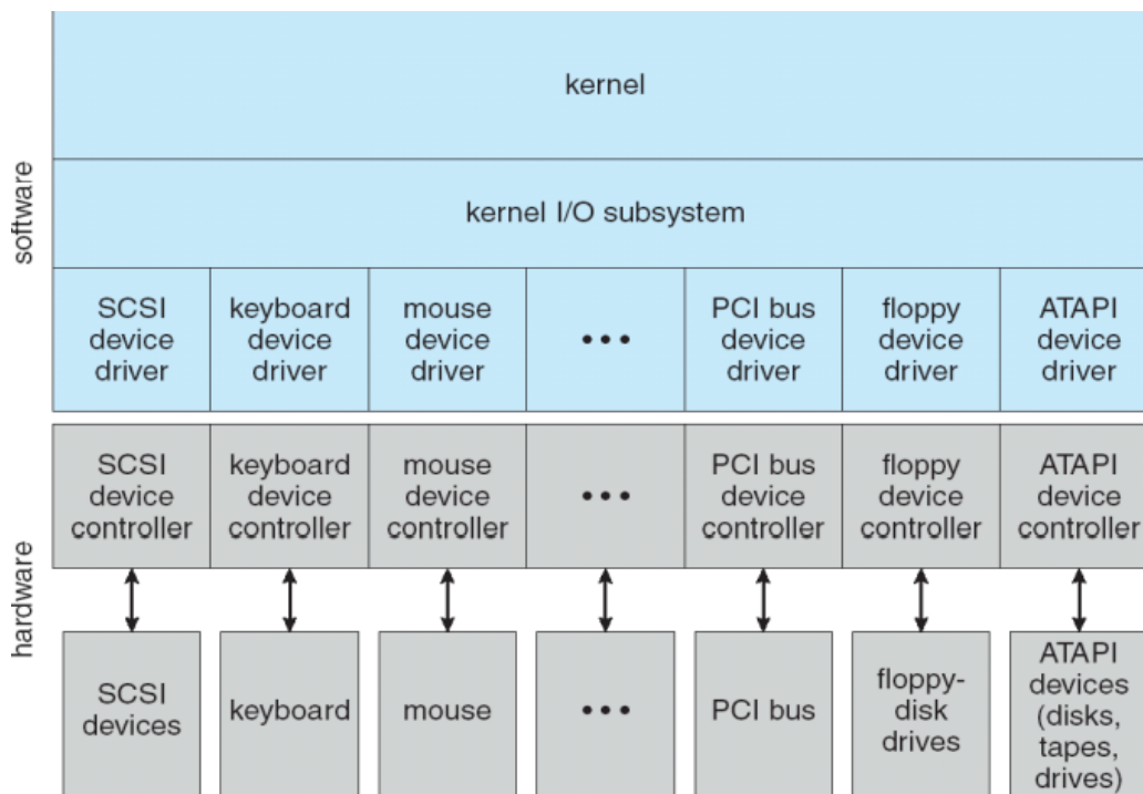
Figure 17.5 A kernel I/O structure
