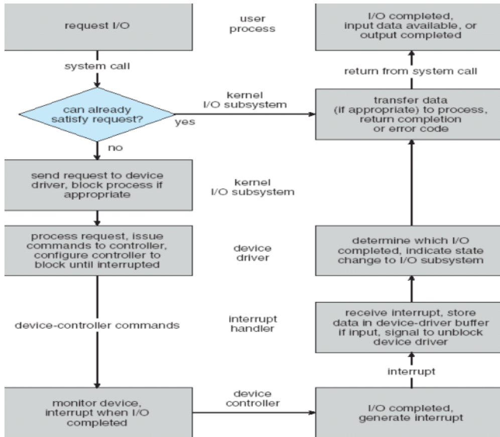
Figure 17.9 The life cycle of an I/O request
