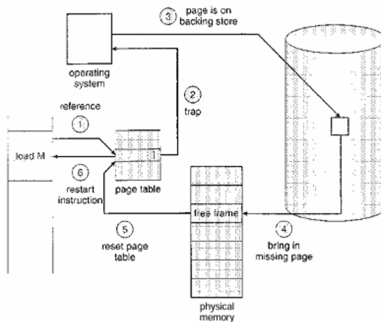
Figure 13.6 Steps in handling a page fault
