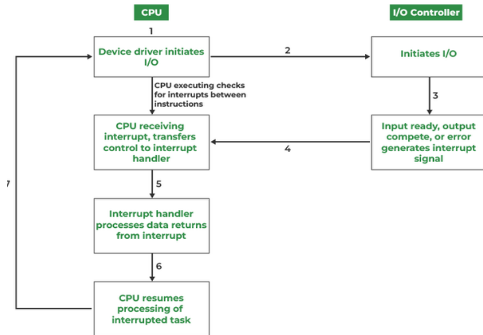
Figure 17.3 Interrupt-driven I/O cycle.
