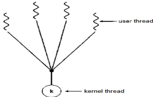
Figure 5.2 Many-to-one model
