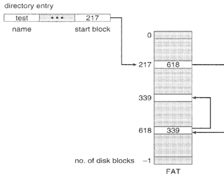
Figure 15.7 File-allocation table
