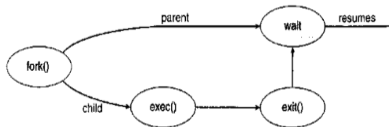
Figure 3.11 Process creation.
