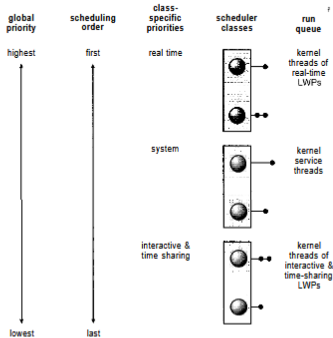
Figure 7.3 Solaris Scheduling
