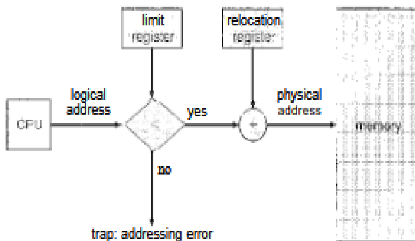
Figure 11.3 Hardware support for relocation and limit registers
